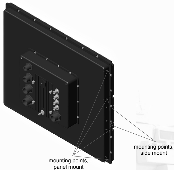
Figure 3-1: Mounts
