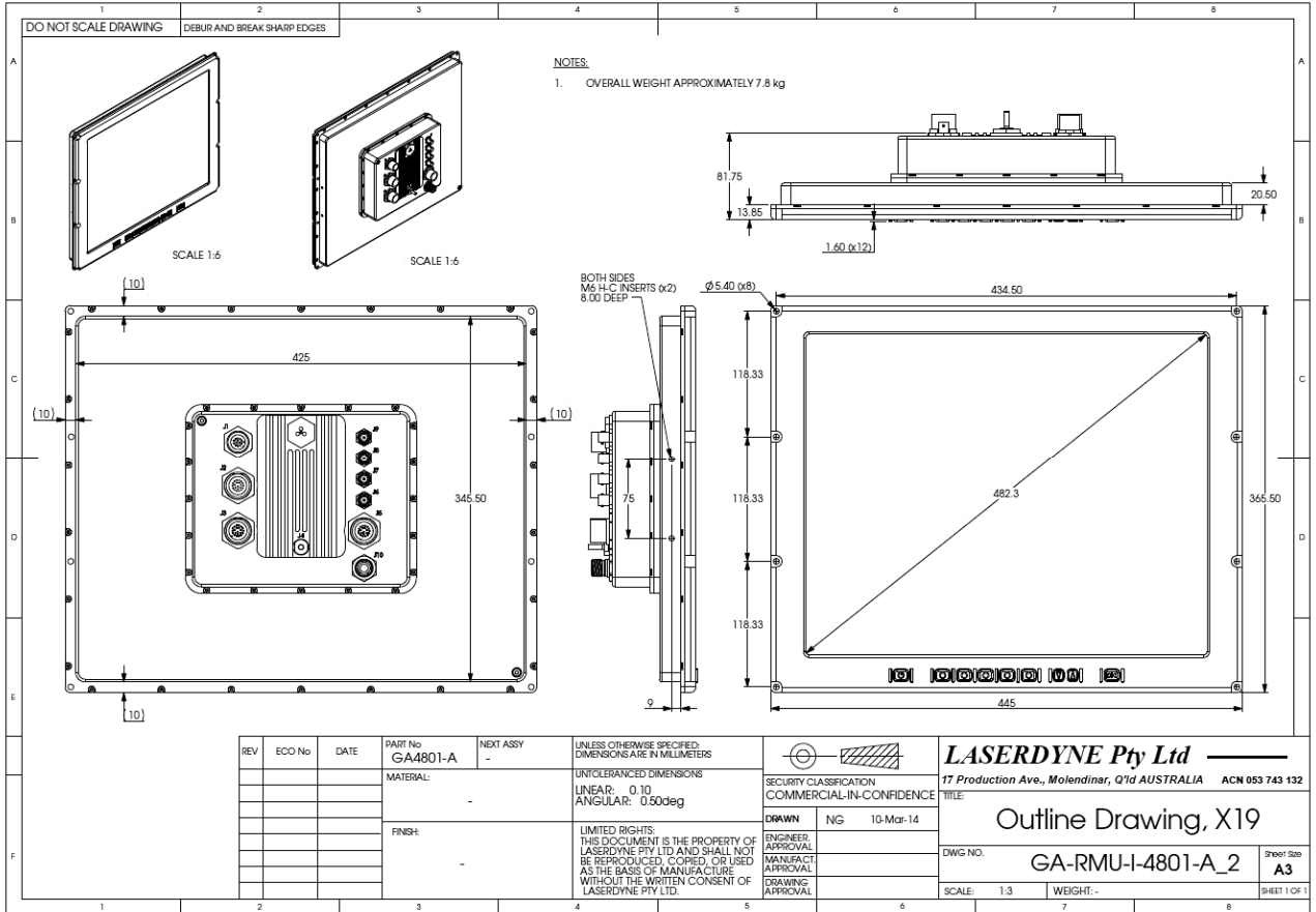
Figure 4-1: Outline Drawing
