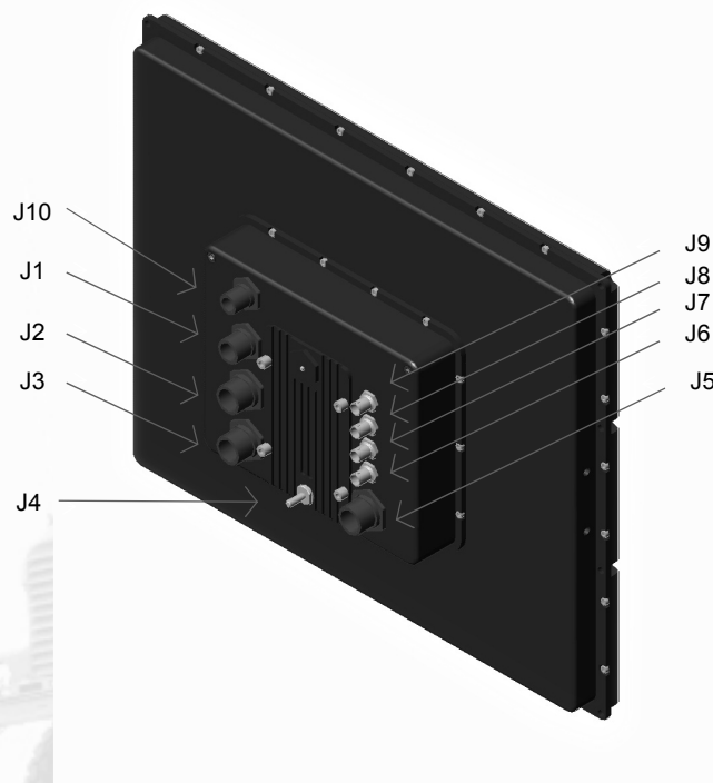
Figure 3-2: Connections
