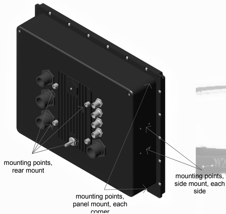
Figure 3-1: Mounts
