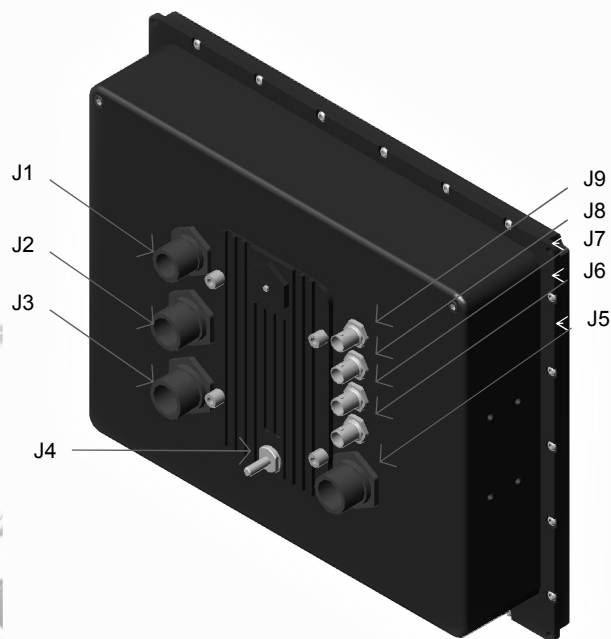
Figure 3-2: Connections
